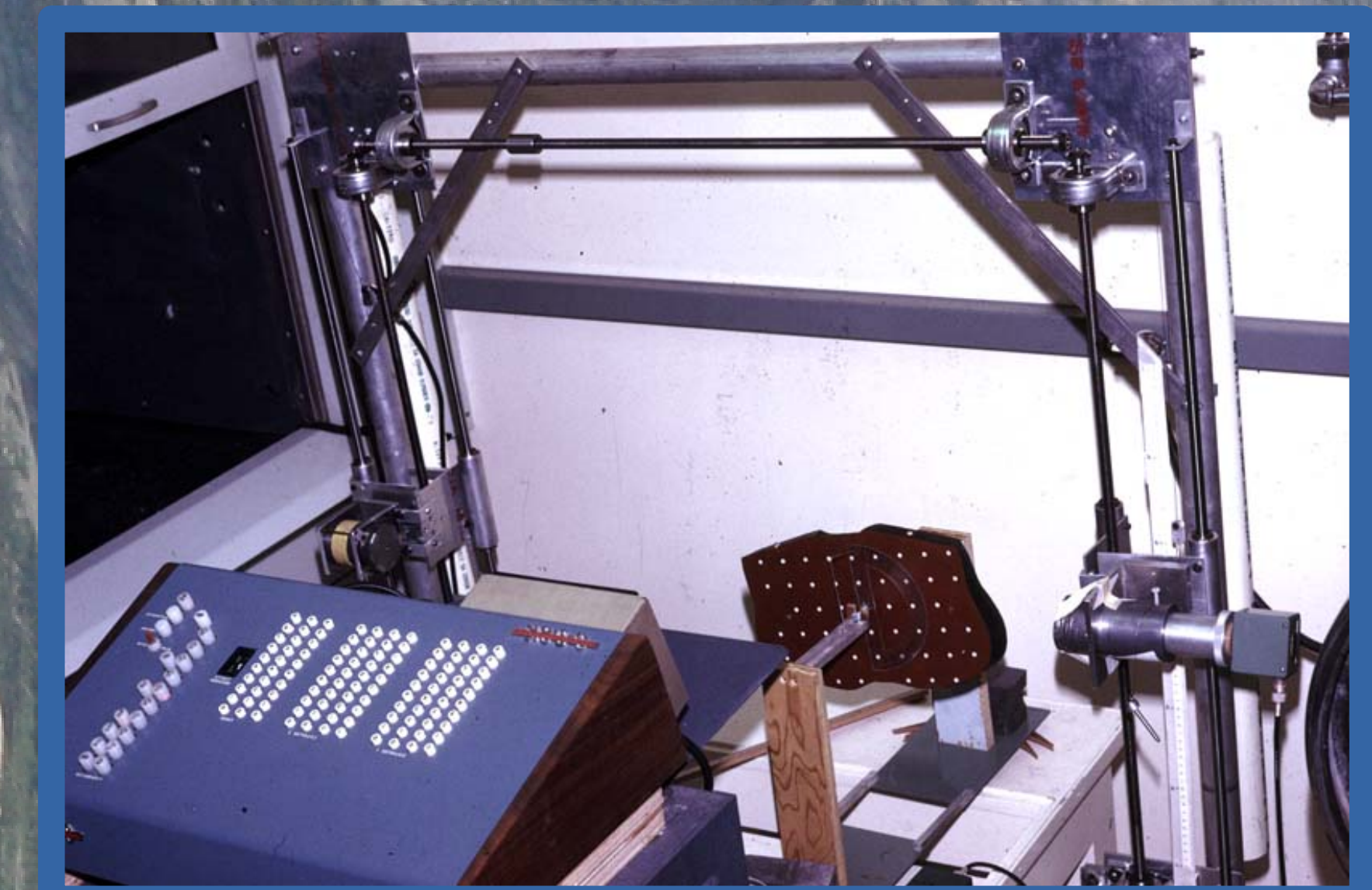
First MeV CT-simulator
