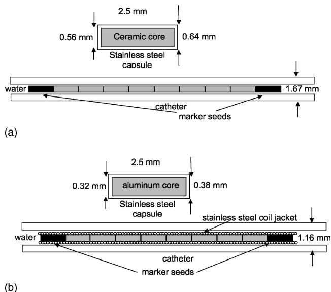
FIG. 2. Schematic showing (a) 5 F single seed of ^{90}\text{Sr}/^{90}\text{Y} and an 8-seed train with gold markers on the ends, and (b) 3.5 F single seed of ^{90}\text{Sr}/^{90}\text{Y} and an 8-seed train with Pt/Ir markers at the ends in a stainless steel wire jacket.
